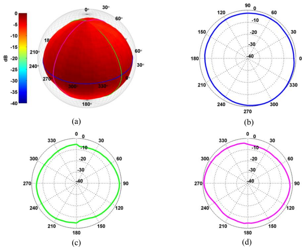
Figure 6.2. Violin directivity of the fundamental frequency for a Bb3. (a) Directivity balloon. (b) Directivity in the transverse plane. (c) Directivity in the medial plane. (d) Directivity in the frontal plane.
